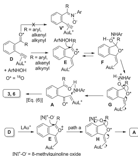
Scheme 2. Proposed reaction mechanism.
