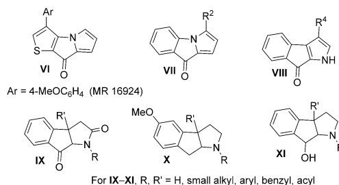
Figure 1. Bioactive indene molecules containing nitrogen.
